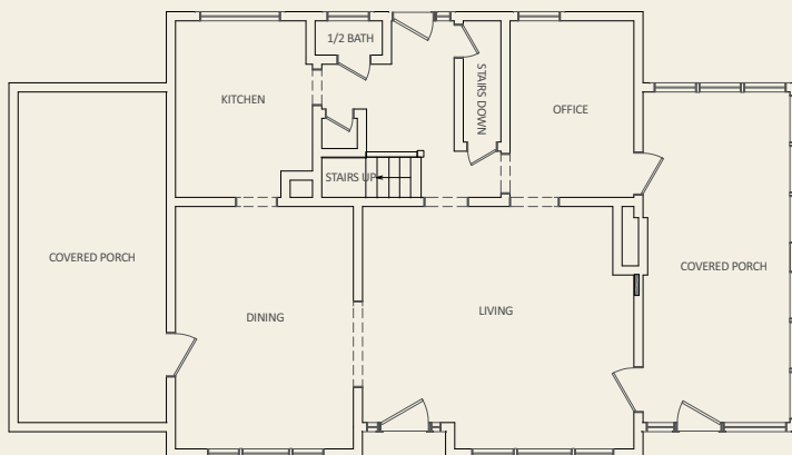
ORIGINAL FLOOR PLAN
