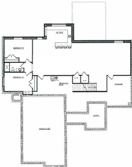
FOUNDATION PLAN
